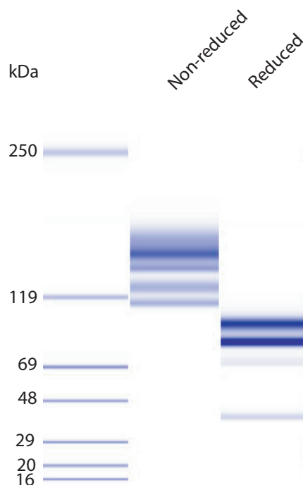
Figure 1. LabChip analysis of Wnt Surrogate-Fc Fusion Protein
