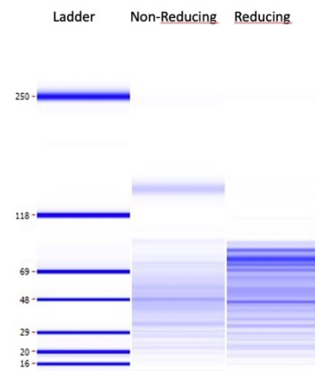
Figure 1 LabChip Capillary Electrophoresis of N002, lot 7328
